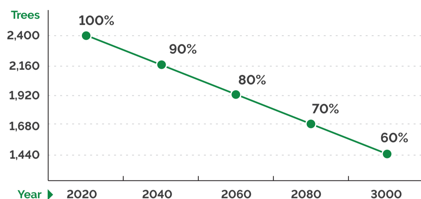
Approximate projection of coco de mer population
